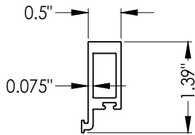
3 PANEL STOP
