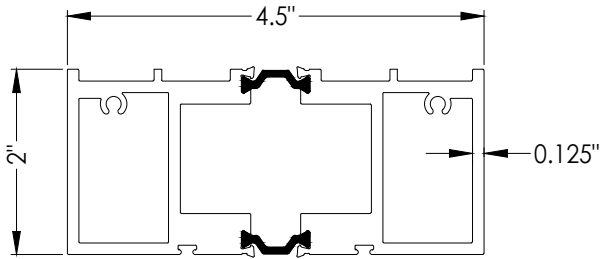
1 HEAD
