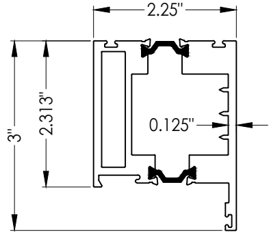
4 TOP RAIL
