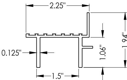
8 SUB SILL
