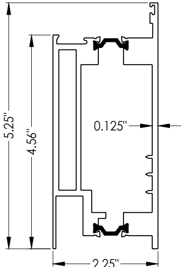
5 BOTTOM RAIL
