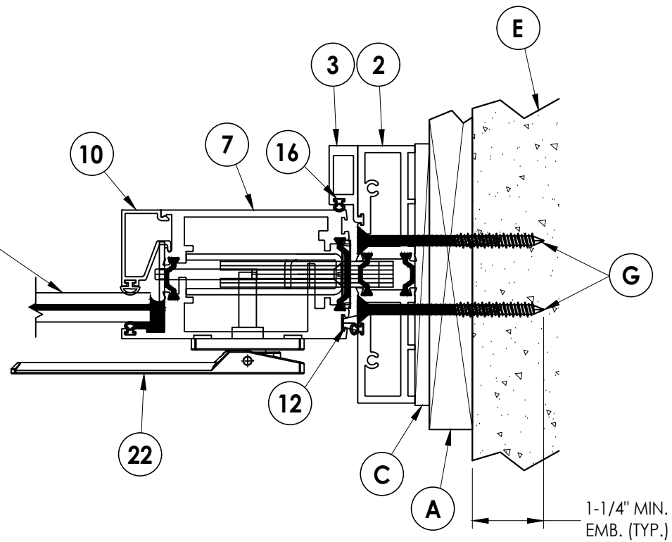
2 HORIZONTAL CROSS SECTION 3 1X Buck Construction
